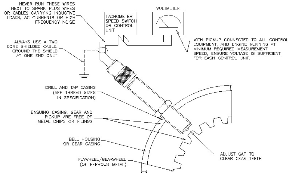
TYPICAL INSTALLATION
